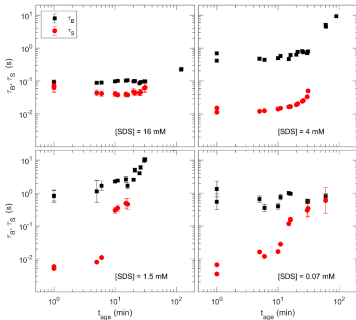
Figure 6. evolution of Brownian decay time \tau_B and shear decay time \tau_S as a function of the ageing time of the emulsion, for emulsions stabilized by different [SDS] content. At long ageing times, \tau_S cannot be precisely determined once Brownian diffusion dominates and \tau_B > \tau_S ; the fit yields a value of \tau_S that lies outside of the axis's limits.
