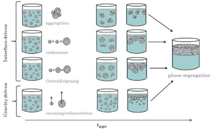
Figure 1: mechanisms determining emulsions destabilization: creaming, coalescence, and Ostwald Ripening.
