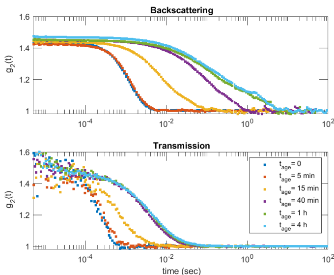
Figure S4. DWS measurements on dodecane-in-water (50/50) emulsions stabilized by [SDS] = 4\text{mM} , performed using the laboratory equipment of the Soft Matter Dynamics instrument. Emulsification was performed by pulsing the piston of the sample cell at 10Hz for 2 min. Note the change of the shape of the correlation function as the emulsion ages, indicating a transition from the ballistic dynamics characteristic of creaming ( t_{\text{age}} < 5\text{ min} ) to Brownian diffusion (15 – 40min), and then to arrested dynamics typical of a crowded environment (1 – 4 hours).
