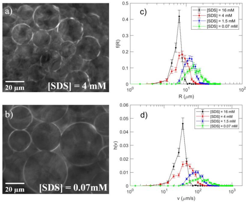
Figure 3. Microscopy images showing individual drops from dodecane-in-water (50/50 volume ratio) emulsions stabilized by SDS in concentration [SDS] = 4 mM (panel a) and 0.07 mM (panel b). c) Distributions f(R) of drop radii of emulsions for different contents of surfactant, deduced from images of representative ensembles of at least 350 individual drops d) Distributions h(v) of creaming velocities, calculated according to Hadamard-Rybczynski equation (1) from the drop radii distributions f(R) of panel c);
