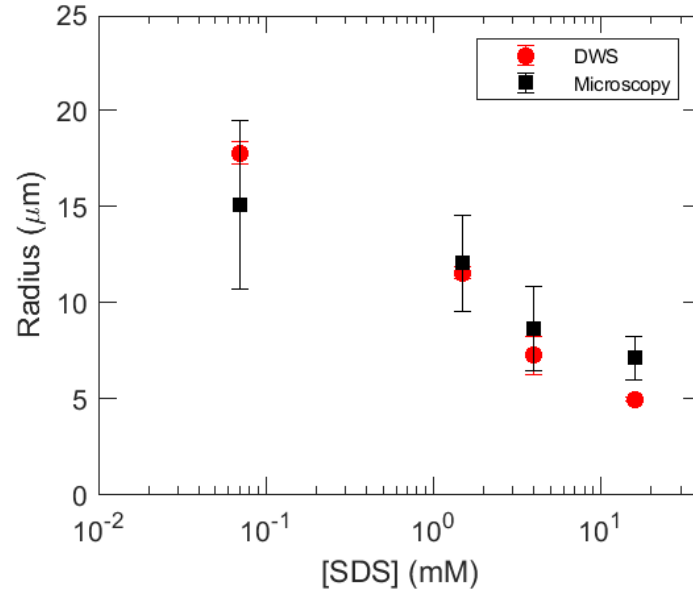
Figure 5. mean drop radius of freshly prepared emulsions as a function of [SDS], as deduced from the transport mean free path l^* according to ray-tracing simulations [40] (red circles) and from direct microscopy observation (black squares). In the case of Microscopy, error bars represent the actual width of the drop radii distribution. In the case of DWS instead, the width of the distribution is not directly accessible, and the error bars are statistical uncertainties.
