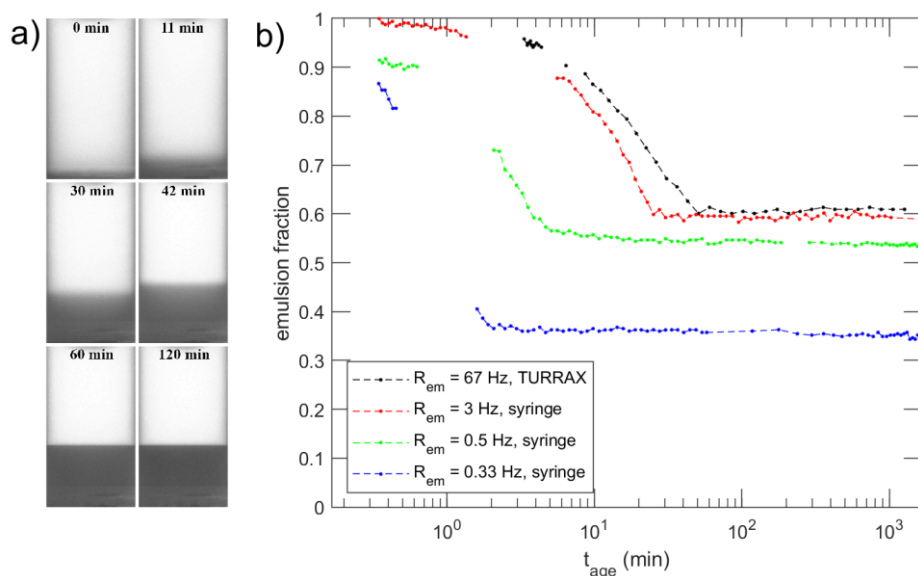
Figure S2. a) Creaming process in a dodecane-in-water (40/60 volume ratio) emulsion stabilized by [SDS] = 4\text{ mM} and produced by UltraTurrax mixing. b) Relative height of the emulsion reported as a function of ageing time, for dodecane-in-water (40/60) emulsion with [SDS] = 4\text{ mM} produced at different emulsification rates by UltraTurrax mixing (black, corresponding to the images in panel a) and syringe extrusion (colours). Time zero corresponds to the end of the preparation process, which includes pouring the emulsion in the cuvette.
