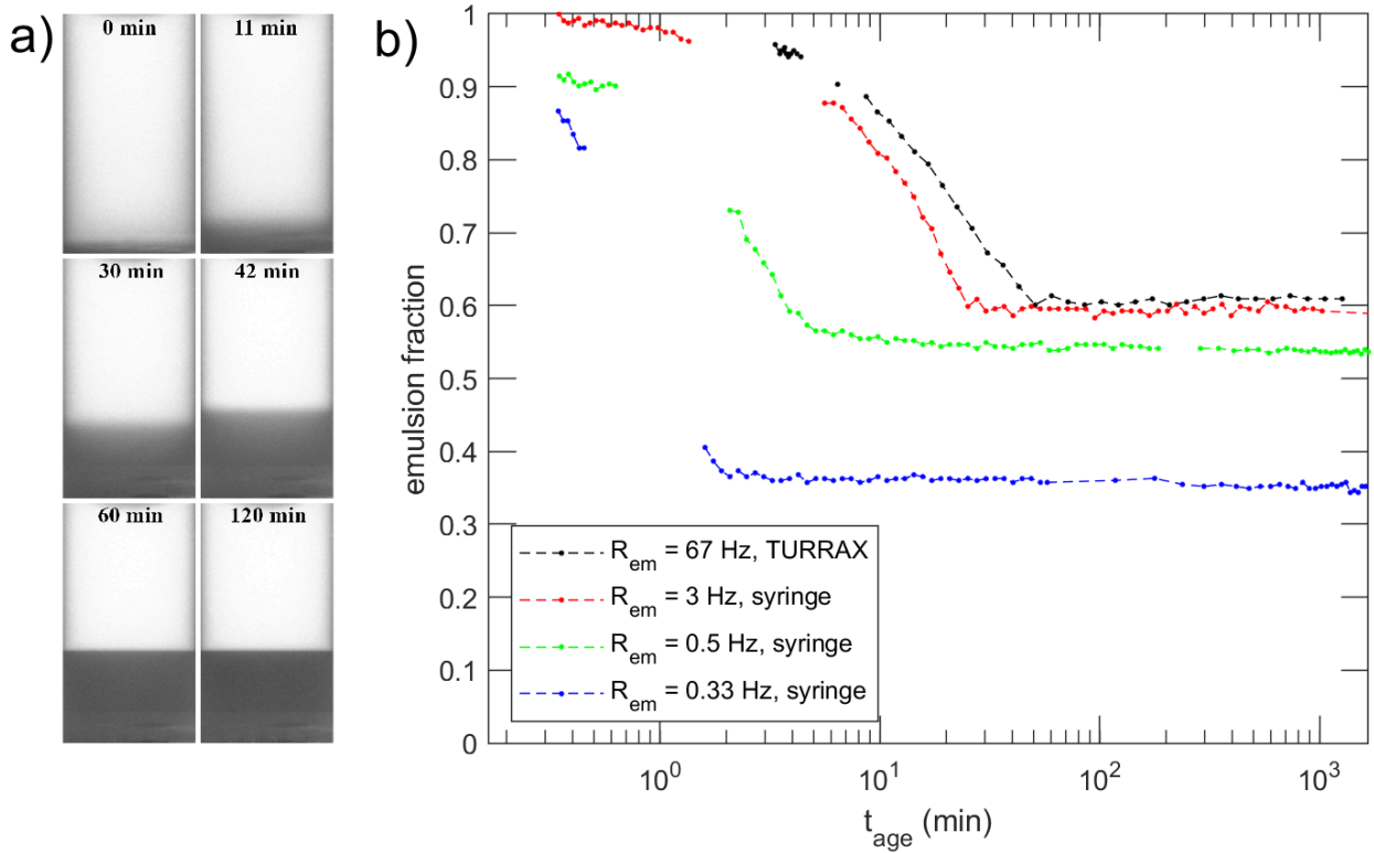
Figure S2. a) Creaming process in a dodecane-in-water (40/60 volume ratio) emulsion stabilized by [SDS] = 4 mM and produced by UltraTurrax mixing. b) Relative height of the emulsion reported as a function of ageing time, for dodecane-in-water (40/60) emulsion with [SDS] = 4 mM produced at different emulsification rates by UltraTurrax mixing (black, corresponding to the images in panel a) and syringe extrusion (colours). Time zero corresponds to the end of the preparation process, which includes pouring the emulsion in the cuvette.
