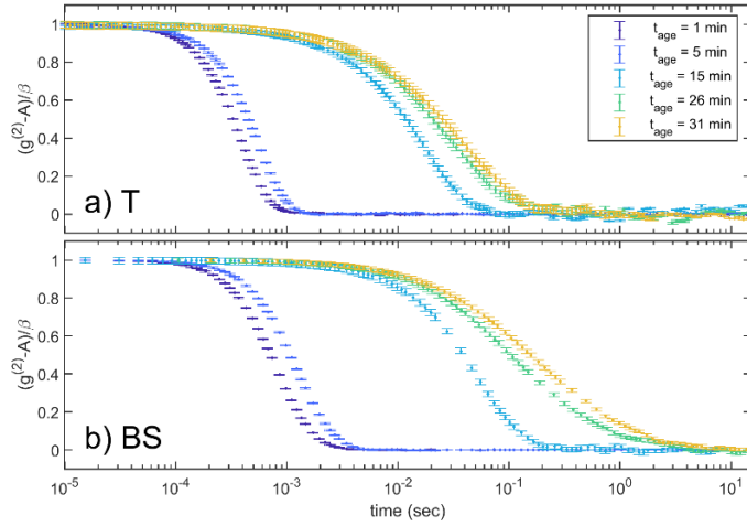
Figure 4. DWS Transmission (T, panel a) and Backscattering (BS, panel b) correlation functions, simultaneously measured on a freshly prepared dodecane-in-water (50/50 volume ratio) emulsion stabilized by SDS at the concentration 1.5 mM. Correlation functions decay with a compressed shape at short ageing time; as the creaming process ends, the correlation functions decay more slowly and with a less steep shape, suggesting the transition from ballistic to Brownian dominated dynamics.
