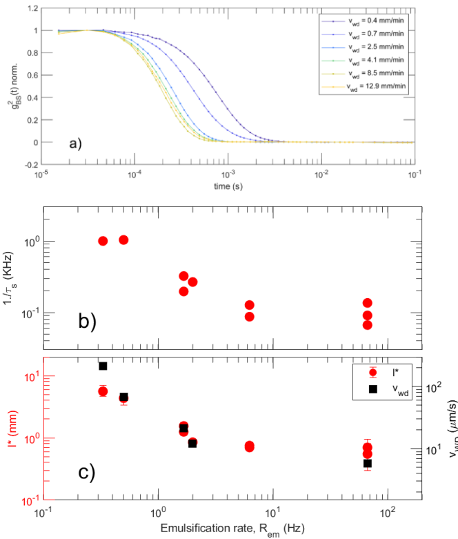
Figure S3. DWS measurements on creaming emulsion as a function of the average water drainage speed v_{wd} determined from macroimaging measurements. a) normalized multispeckle backscattering correlation function; all have a compressed exponential shape, indicating \tau_S \ll \tau_B . b) inverse of the shear decay time \tau_S decreases as a function of the emulsification rate R_{em} , indicating a reduction in the width of the velocity distribution as the emulsification energy is increased. c) l^* (left axis) and the average drainage speed v_{wd} (right axis) scale in the same fashion as a function of R_{em} ; the two y-axes span equal logarithmic intervals.
