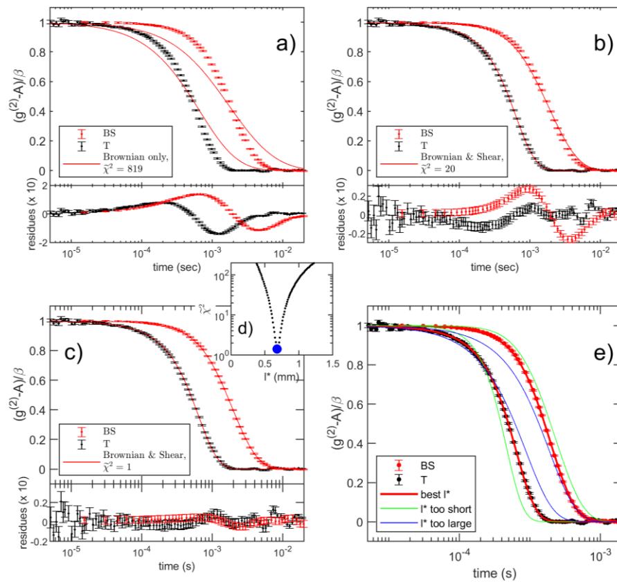
Figure 2. DWS correlation functions measured in transmission (T, black points) and backscattering (BS red points) on a dodecane-in-water emulsion (50/50 volume ratio) stabilized by SDS surfactant (4 mM) at t_{age} = 10 \text{ min} . Errorbars are deduced by the method reported in [5]. a) Fit with the classical analytical model of eq. 5 and 6, assuming purely Brownian dynamics; the very high value of \chi^2 and the residue plot (inset at the bottom) indicate that this model badly fails. b) Fit with an analogous analytical model, now
