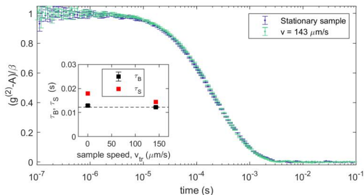
Figure S1. Comparison of DWS measurements performed on 1 \mu\text{m} polystyrene nanoparticle suspension, stationary and under uniform translation in the vertical direction at 143 \mu\text{m/s} . The inset report the relaxation times obtained by the fitting procedure described in
