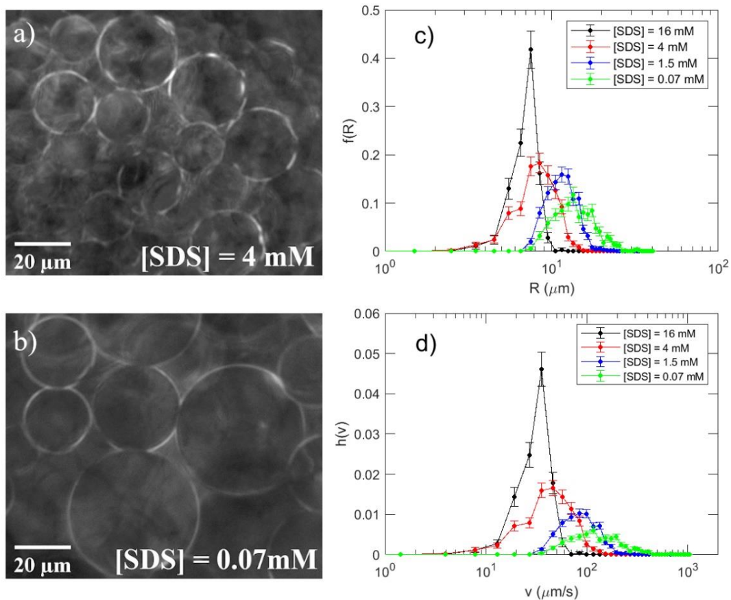
Figure 3. Microscopy images showing individual drops from dodecane-in-water (50/50 volume ratio) emulsions stabilized by SDS in concentration [\text{SDS}] = 4 \text{ mM} (panel a) and 0.07 \text{ mM} (panel b). c) Distributions f(R) of drop radii of emulsions for different contents of surfactant, deduced from images of representative ensembles of at least 350 individual drops d) Distributions h(v) of creaming velocities, calculated according to Hadamard-Rybczynski equation (1) from the drop radii distributions f(R) of panel c);
