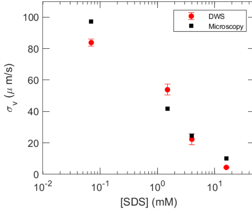
Figure 7. Comparison of the standard deviation of velocities, \sigma_v , measured at early times as a function of surfactant content [SDS] by DWS (red circles), with the same quantity obtained from the Hadamard-Rybczynski relation (eq. 1), assuming the drop size distribution measured by microscopy (black squares).
