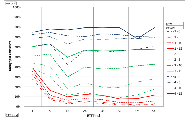
Figure 16: Throughput efficiency vs RTT. NTN-CDL NLOS channel, speed 100 km/h, FER \leq 10^{-2} .
