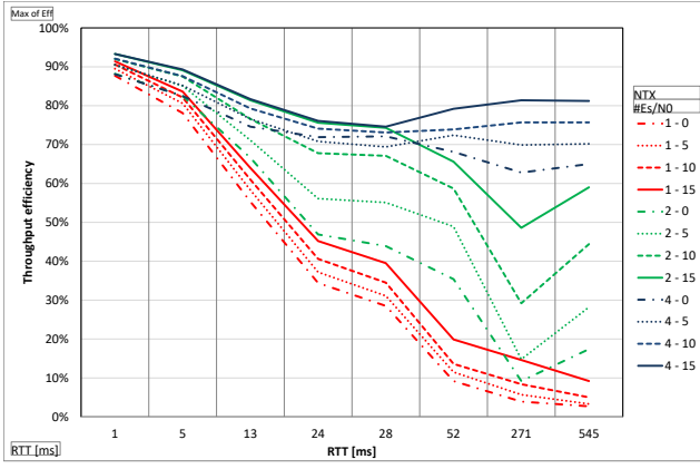
Figure 15: Throughput efficiency vs RTT. NTN-CDL NLOS channel, speed 10 km/h, FER \leq 10^{-2} .
