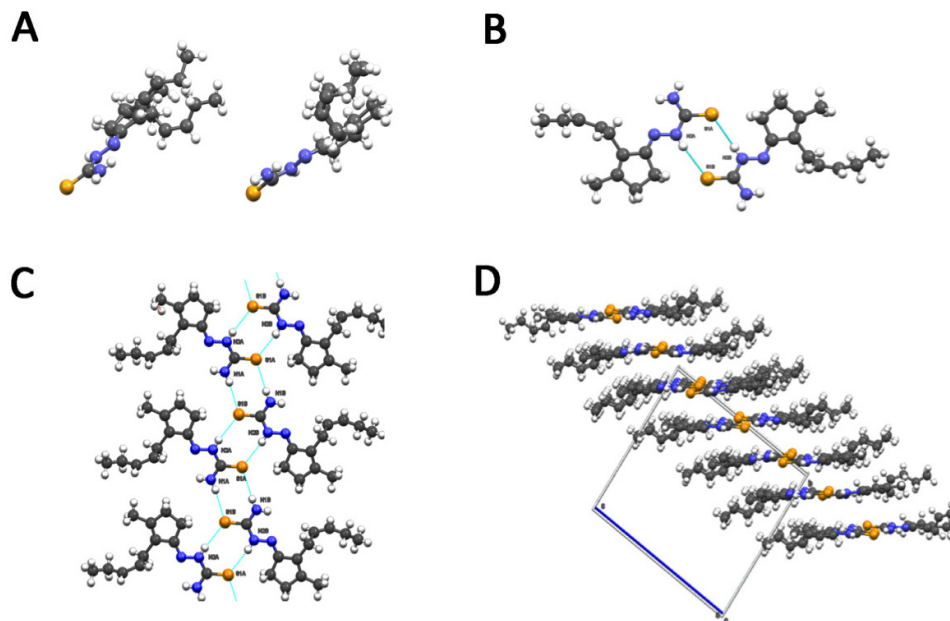
Figure 1. (A) Overlapping of molecules A/B (left) and A/C (right). (B) Hydrogen bonding scheme between molecule A and B. (C) Hydrogen bond scheme along the ribbons formed by molecules A/B. (D) packing of the ribbons. Sulfur is represented in yellow, nitrogen in blue and carbon in gray.
