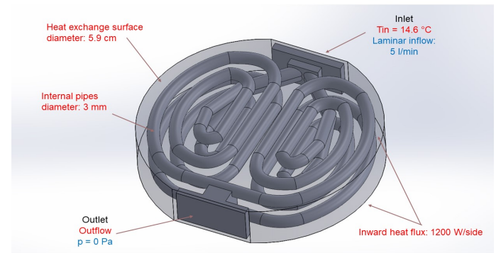
Fig. 9. 3D model of the inner layout of the “Ram” cold plate and simulation operative conditions.
