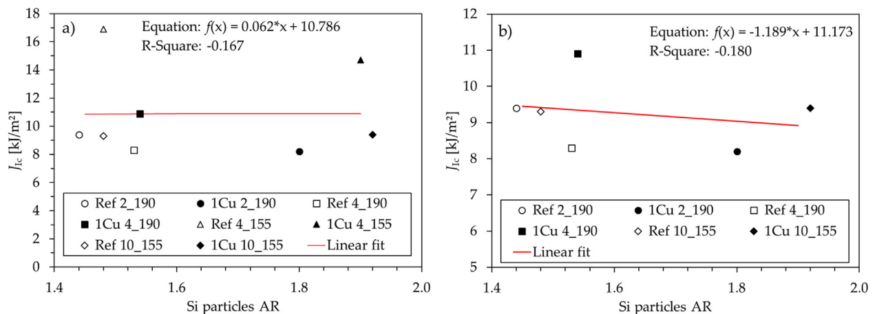
Fig. 12 – Fracture toughness vs. Silicon particles aspect ratio (AR). In (a) for all data results and in (b) without the data results of the heat-treated specimens by 4 h at 155 °C.
