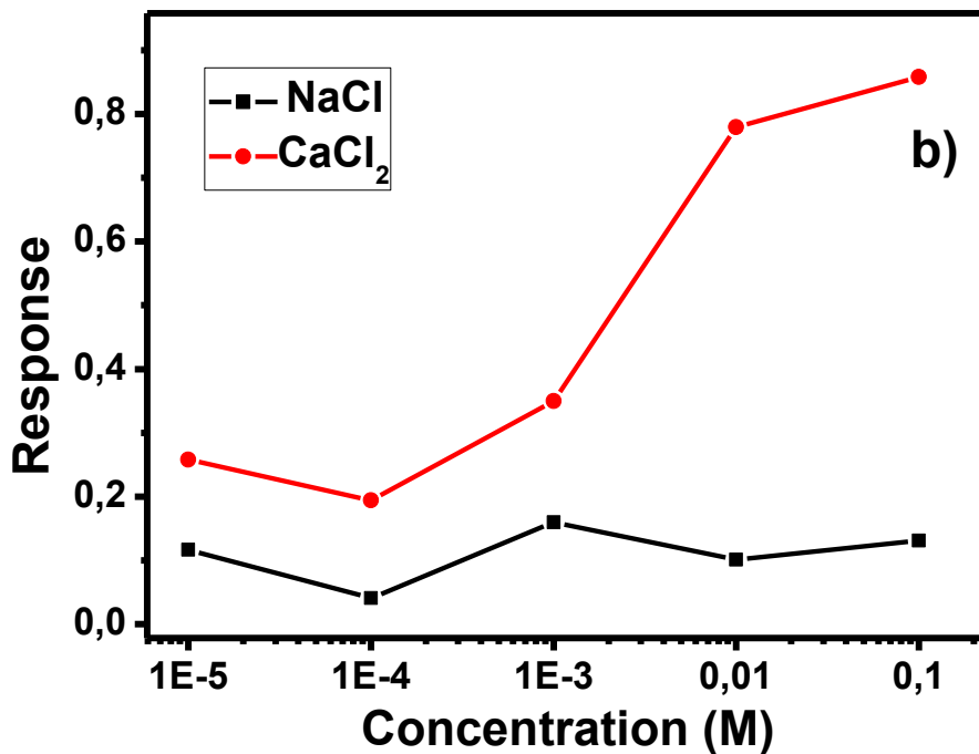
Figure 4: Comparison between responses obtained with \text{CaCl}_2 and \text{NaCl} solutions on calcium-selective textile OECT; a) Response as a function of gate voltage from 0.2 to 1 V with 0.2 V step for different concentration of \text{NaCl} (green tones) and \text{CaCl}_2 (red tones) from 10^{-5}\text{M} to 10^{-1}\text{M} ; b) Responses at 1 V V_g as a function of \text{NaCl} and \text{CaCl}_2 concentrations
