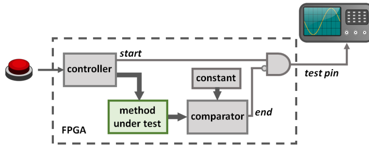
Figure 8. Measurement set-up for the field programmable gate array (FPGA) platform.
