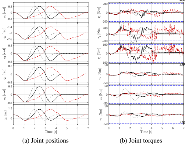
Figure 4: Comparison of measured joint positions and torques for Task B. Dashed gray line: nominal reference. Solid black line: QP-PTS-IB method. Dash-dot red line: non-predictive scaling method. Dashed blue line: torque limits.
