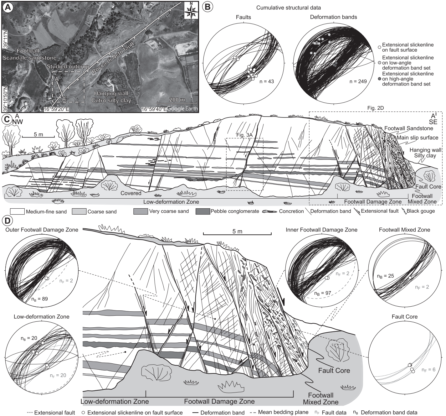
Figure 2. (A) Satellite image (Google Earth) of the investigated Rocca di Neto fault zone (Crotona Basin, Southern Italy) with the trace of the master fault and the position of the studied outcrop. (B) Cumulative structural data regarding faults and deformation bands through the footwall of the Rocca di Neto fault zone (Schmidt lower hemisphere projection). (C) Detailed geological cross-section of the fault zone with the identified structural domains. (D) Detail of the fault domains, with stereonet plots plotting the structural data (Schmidt lower hemisphere projection).
