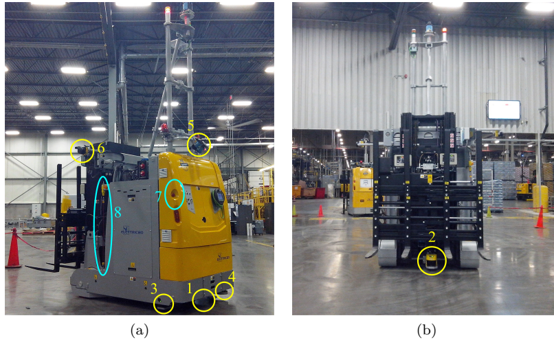
Figure 1: On board safety laser sensors (yellow circles) and emergency stop devices (cyan ellipsoids) of a LGV (Courtesy of Elettric80)
