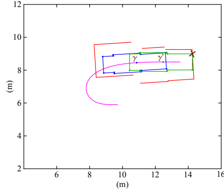
Figure 6: Most critical collision point for the \gamma experiment on curve ID 2.
