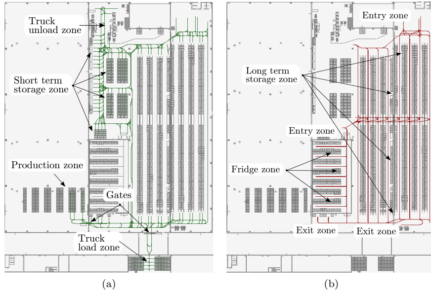
Figure 10: Plant layouts for the CB12 vehicles (a) and for the LT3 vehicles (b).
