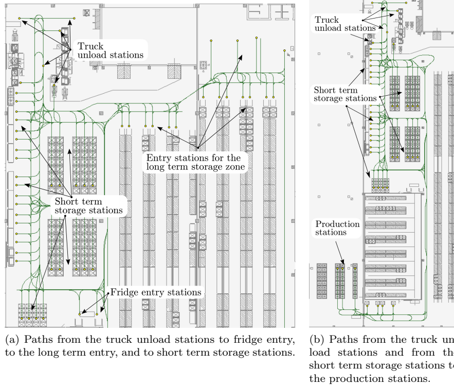
Figure 11: Travel categories 1 (a) and 2 (b).
