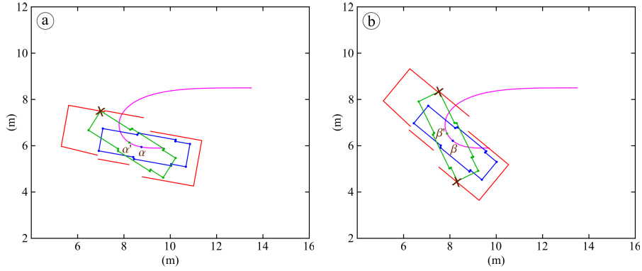
Figure 5: Most critical collision points for the \alpha and \beta experiments on curve ID 2.
