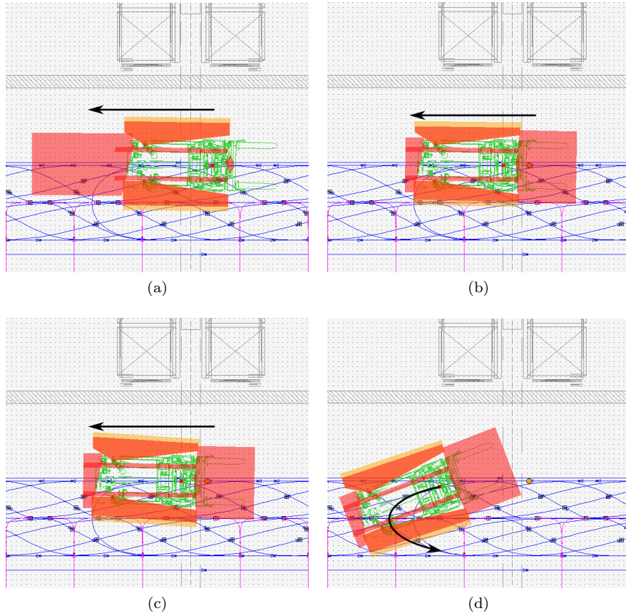
Figure 2: LGV safety areas could be modified only when the vehicle switch between two subsequent segments.
