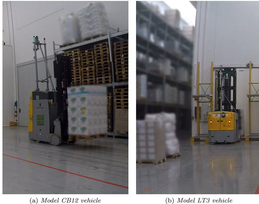
Figure 9: The two LGV models used in the industrial plant considered. (Courtesy of Eletic80).
