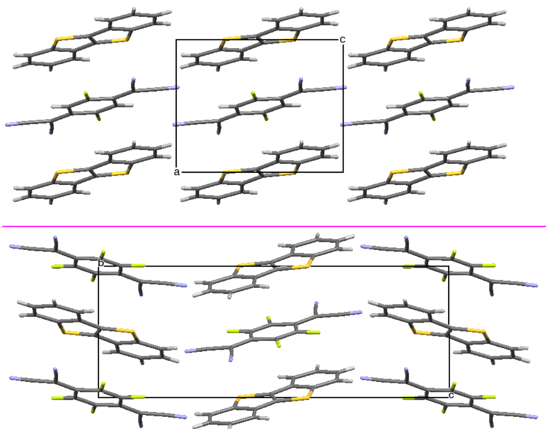
Figure 1. (Top) Crystal structure of BTBT-TCNQF 2 viewed from the b axis. (Bottom) Crystal structure of BTBT-TCNQF 4 viewed from the a axis. The chosen view puts in evidence the stack structure and the three dimensional stack arrangement.
