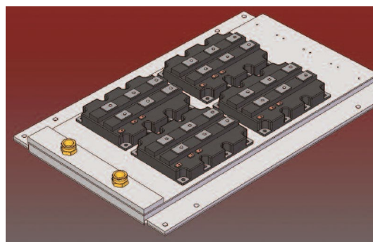
Fig. 1. 3D model of a cold plate with four IGBT modules mounted on it.
