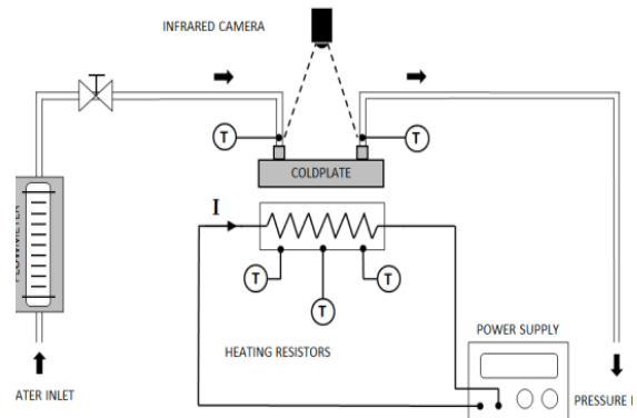
Fig. 5. Schematic of the experimental set-up used for the thermal characterization of the testing cold plate used for CFD-FEM model validation.
