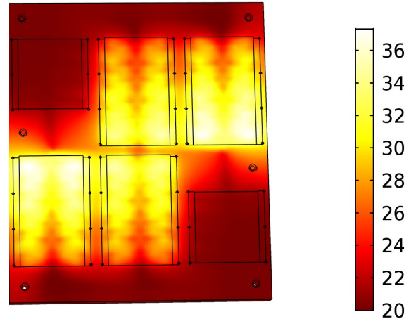
Fig. 9. FEM thermal map simulated after layout optimization by the CFD/FEM-SPICE software tool, for the prototype at the same conditions as in Fig. 7. Color temperature bar in °C.
