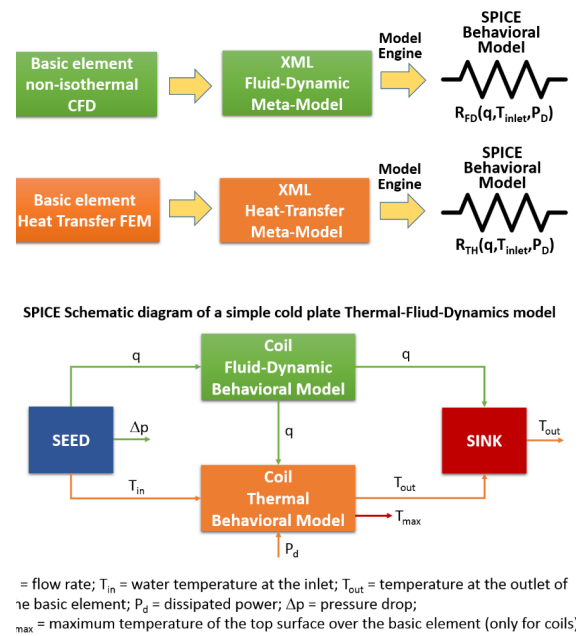
Fig. 2. Schematic diagram of the 3D numerical-SPICE approach for thermo-fluid dynamic simulation of cold plates: (top) basic elements from 3D numerical model to SPICE model transform process; (bottom) SPICE schematic of a simple cold plate.
