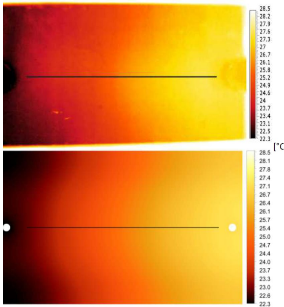
Fig. 6. Testing cold plate surface temperature map measured by IR camera (top) and simulated by the CFD-FEM model (bottom).
