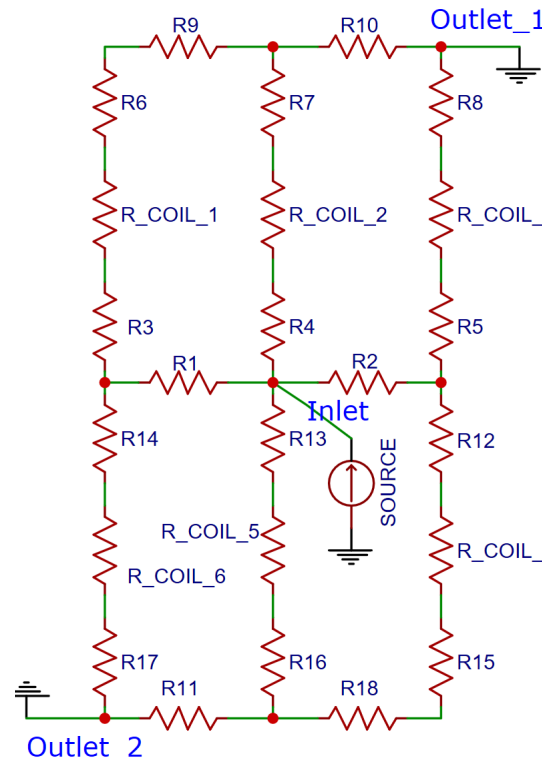
Fig. 8. SPICE equivalent model for the prototype of Fig. 7.
