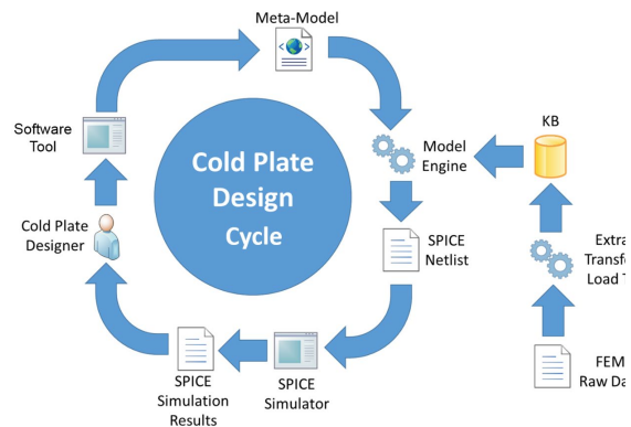
Fig. 3. Flow diagram of the software tool developed to easily exploit the SPICE-CFD/FEM proposed approach for optimized cold plate design.
