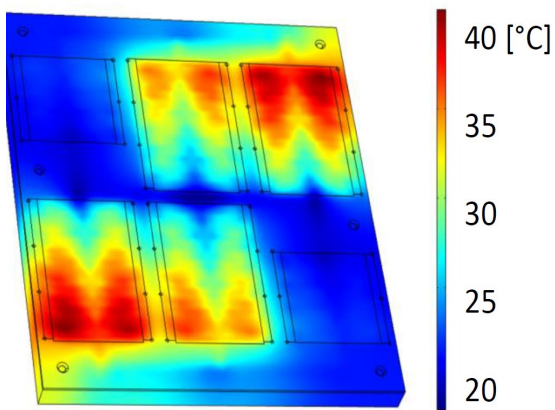
Fig. 7. FEM thermal map for the first design of cold plate for power application, with an input power of 9.1 kW, from 4 IGBT, flow rate of 12 l/min, and inlet water temperature of 20 °C.
