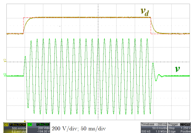
Fig. 17. System response. d-axis voltage v_d and line to line output voltage v .
