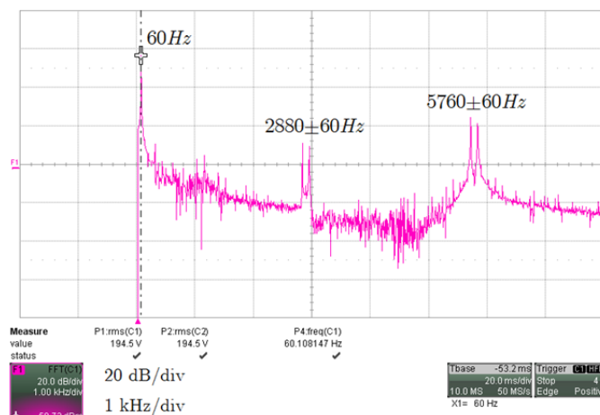
Fig. 18. Line to line output voltage spectrum for the reduced-scale prototype at rated load in single operation.
