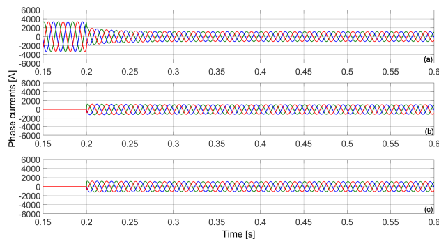
Fig. 16. Slave insertion simulation (at t = 0.2 s) of Master (a) and Slaves (b), (c) output currents, using current sharing control based on PI controller.
