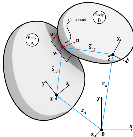
Fig. 1. Bodies A and B in contact; a local reference frame \{\mathbf{n}_i, \mathbf{u}_i, \mathbf{w}_i\} is generated at the contact point based on contact detection information. The contact point is located in the centroidal and principal reference frames via the \tilde{\mathbf{s}}_{i,A} and \tilde{\mathbf{s}}_{i,B} vectors.
