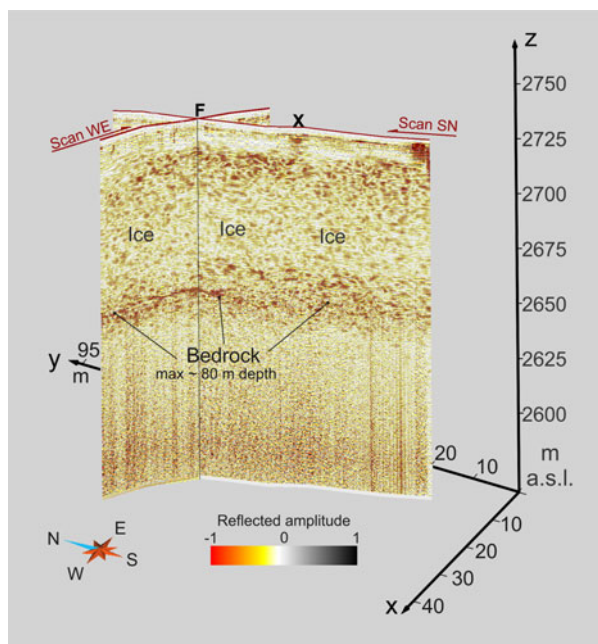
Fig. 8. 3-D representation of the RES depth sections of the Forni glacier (red dotted lines in Fig. 1b). The passive seismic station (F) was located at the intersection of the two RES lines. The X marks scattering from a hidden crevasse.
