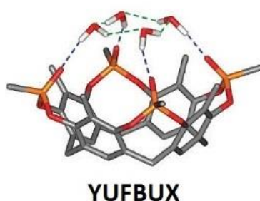
Figure 3.6 Side view of the tetraphosphonate cavitant YUFBUX with the induced cluster of hydrogen-bonded water molecules (Colour code: P, orange; O, red; C, grey; H, white; weak intermolecular interactions, blue and green). Reproduced with permission of The Royal Society of Chemistry from Ref. 90.
