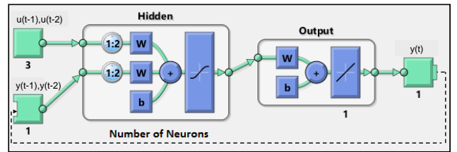
Fig. 2. Closed-loop structure of a single NARX model.
