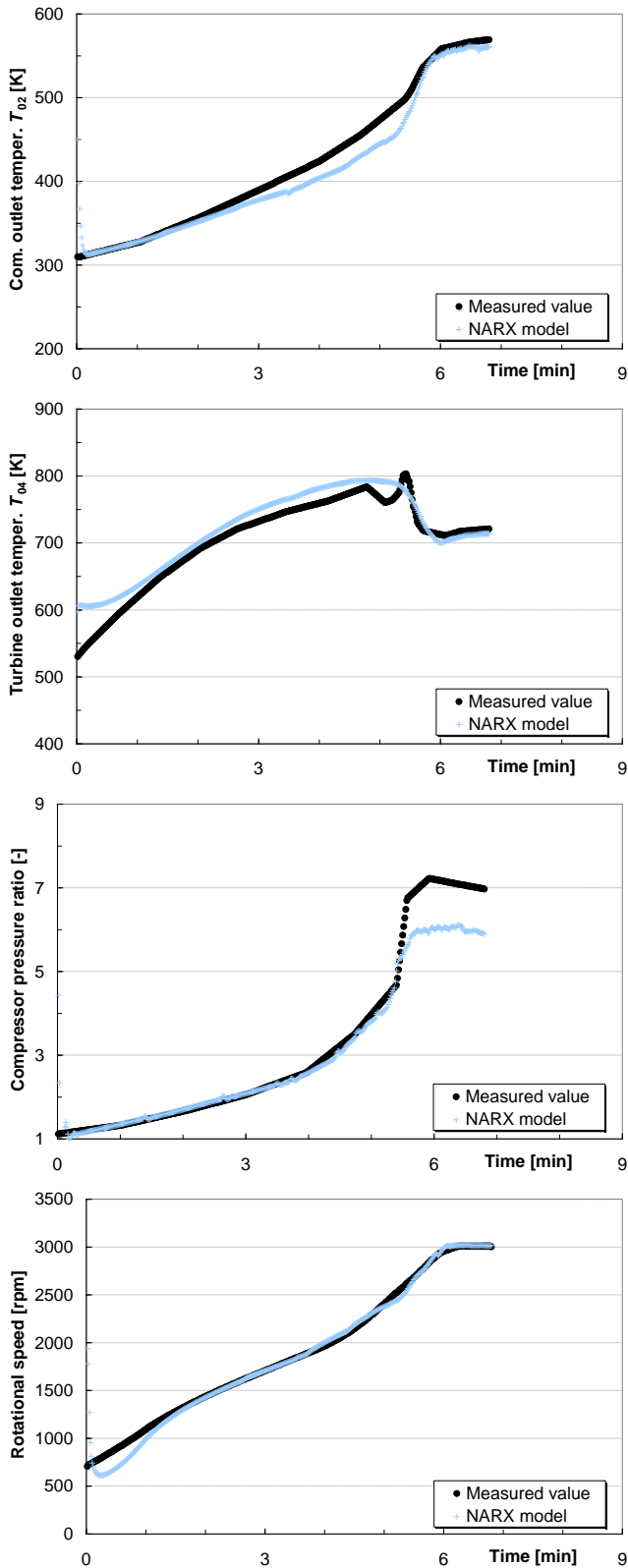
Fig. 11. Variations of compressor outlet temperature T_{02} , turbine outlet temperature T_{04} , compressor pressure ratio P_{cC} and rotational speed N for the testing maneuver TE2.
