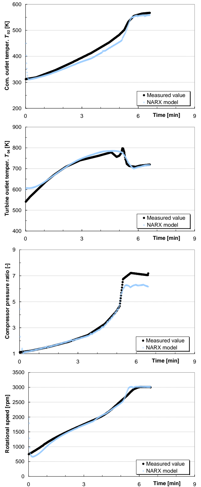
Fig. 12. Variations of compressor outlet temperature T_{02} , turbine outlet temperature T_{04} , compressor pressure ratio P_{cC} and rotational speed N for the testing maneuver TE3.
