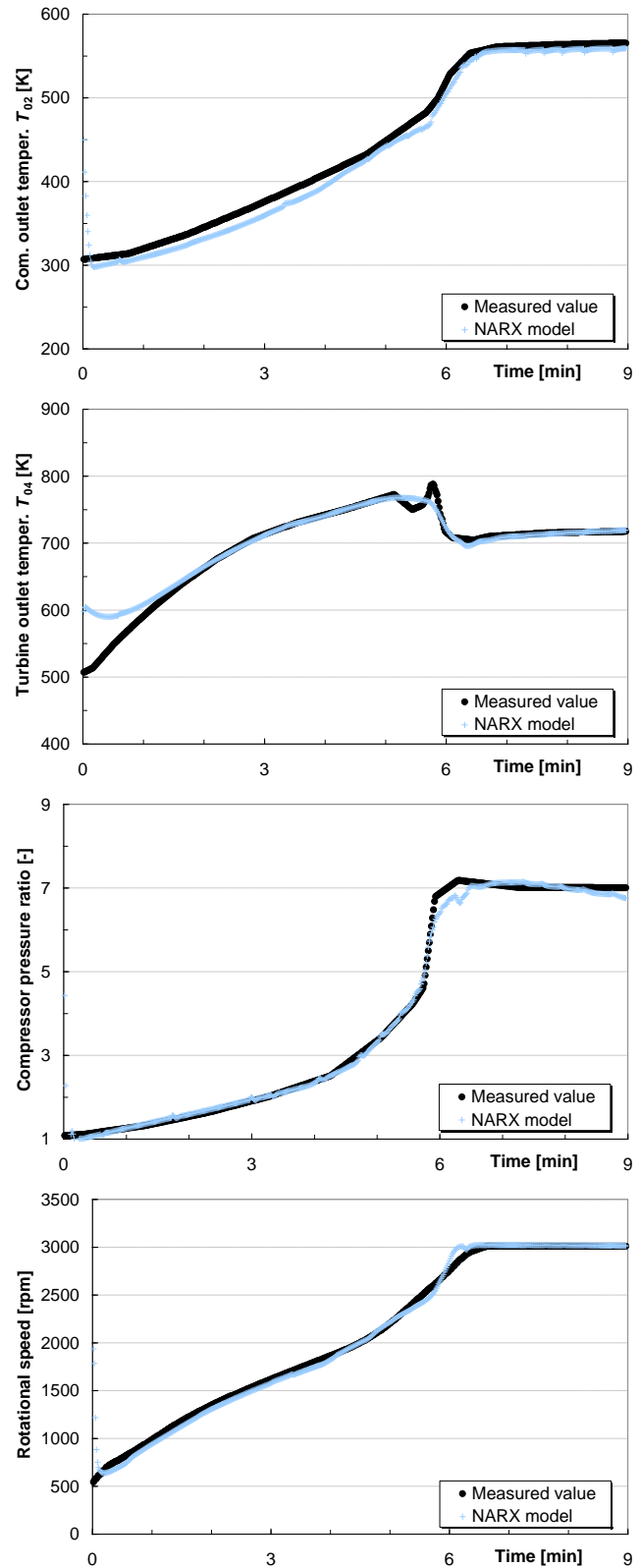
Fig. 10. Variations of compressor outlet temperature T_{02} , turbine outlet temperature T_{04} , compressor pressure ratio P_{rC} and rotational speed N for the testing maneuver TE1.
