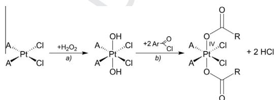
Fig. 2. Synthetic route to prepare complexes 1a–1c (A = NH 3 ) and 2a–2c (A = dach): (a) H 2 O 2 35%, water, RT, 24 h; (b) aryl chloride, acetone, reflux 4 h.
