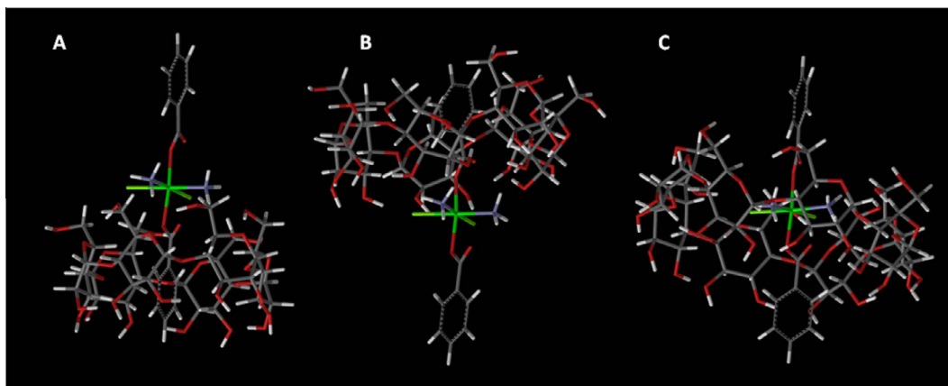
Fig. 7. Minimum energy conformation of the complex between 1a and (A) \alpha -, (B) \beta - and (C) \gamma -CD. CD molecules are oriented with the primary hydroxyl rims in the upper part of the figure whereas the secondary hydroxyl rims are in the lower part of the figure. The models have been obtained by means of molecular modeling calculations.
