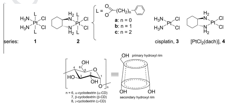
Fig. 1. Sketch of the Pt(IV) complexes under investigation (1a–1c and 2a–2c) and their corresponding Pt(II) parent compounds (3 and 4), along with molecular structures of the cyclodextrins (CDs) under investigation. The CD numbering scheme is reported.
