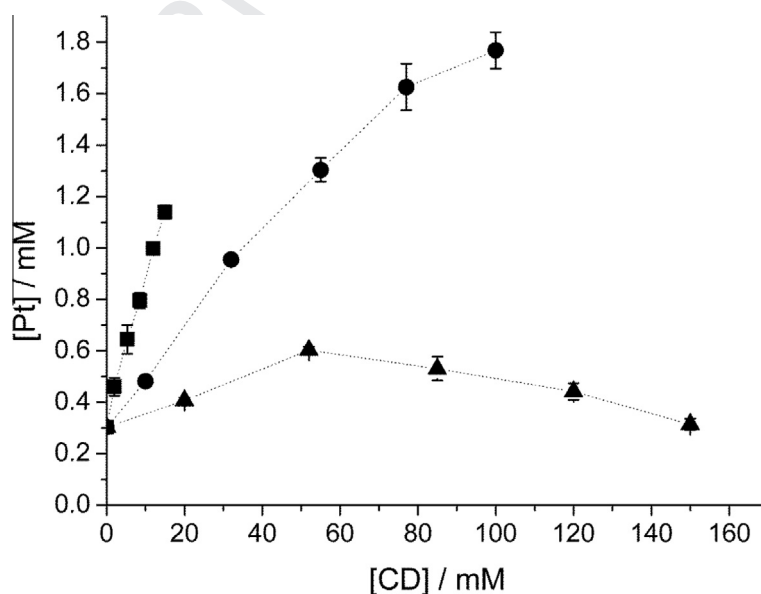
Fig. 5. Phase-solubility diagrams for 1a in the presence of \alpha -(circles), \beta -(squares), and \gamma -CD (triangles) in water solution at 25 °C.
