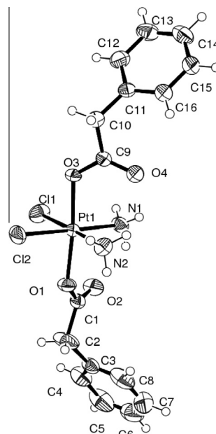
Fig. 3. Ortep plot of compound 1b with ellipsoids at 50% probability.
