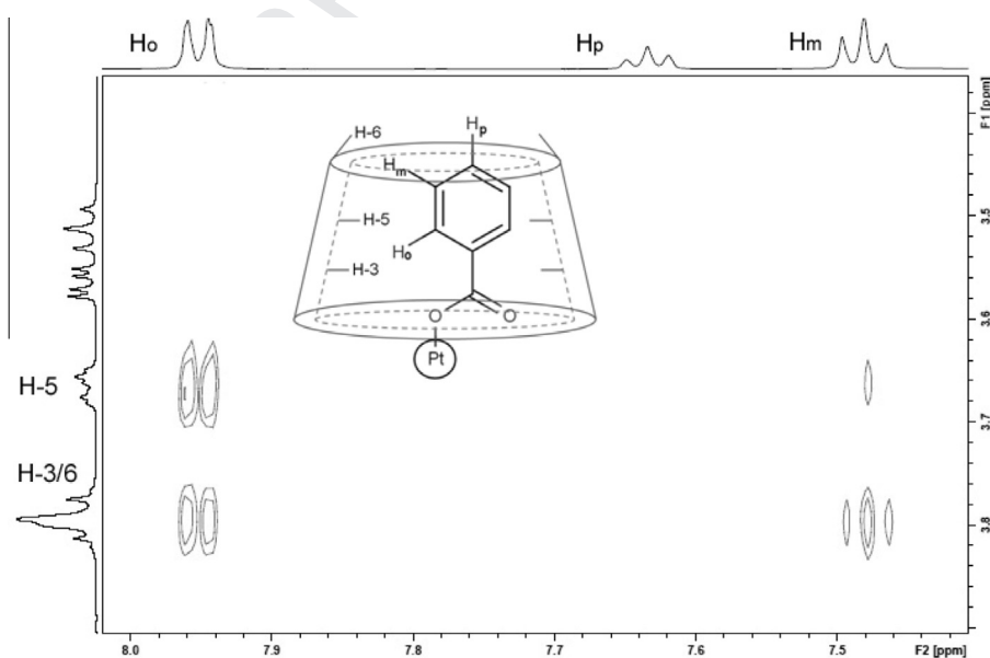
Fig. 6. Expanded region of the ROESY spectrum of 1aCD and proposed geometry for the inclusion of 1a into \beta -CD.
