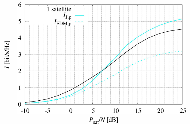
Figure 14. Spectral efficiency achievable by DVB-S2 constellations for two satellites and \gamma^2=-6 dB.
