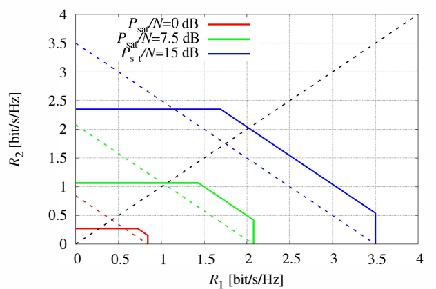
Figure 15. Spectral efficiency regions for DVB-S2 constellations for two satellite transmitting with P_{sat}/N equal to 0, 7.5 and 15 dB and \gamma^2=-6 dB.
