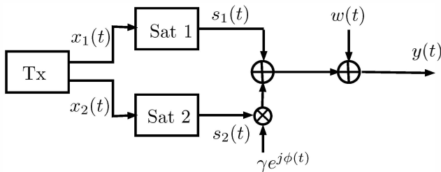
Figure 1. Block diagram of the analyzed system.
