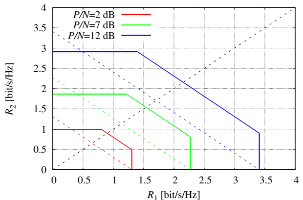
Figure 8. Spectral efficiency regions for \gamma^2 = -2 dB.
