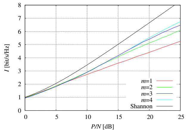
Figure 5. Spectral efficiency for single transmitter (AWGN channel with peak power constraint).
