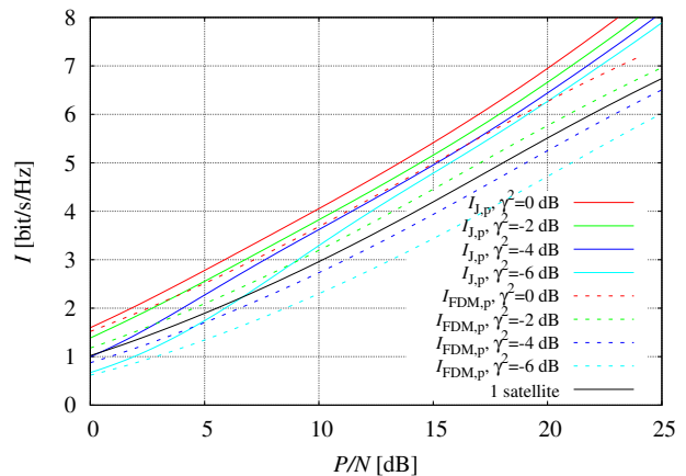
Figure 7. Pragmatic spectral efficiency for different values of \gamma (AWGN channel with peak power constraint).
