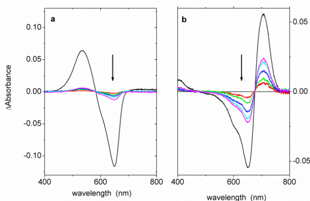
Figure 7 Difference absorption spectra recorded after 500 s illumination steps (total =2550) at 650 nm, starting for the "red" forms of GAF3 (a) and Cph1 (b). The arrow's direction indicates increasing illumination times. Black lines refer to the fully photoconverted forms, i.e. GAF3 G -GAF3 R and Cph1 FR -Cph1 R . T = 20 °C.
