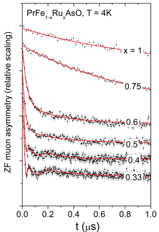
FIG. 5. (Color online) Time dependence of ZF- \mu SR asymmetry for x = 0.33, 0.4, 0.5, 0.6, 0.75 , and 1 at T = 4 K. For graphing purposes, each composition is shifted along the vertical axes by an arbitrary constant.
