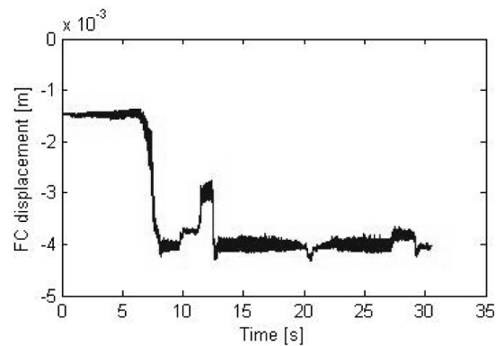
Fig. 20. Flow compensator simulated displacement
