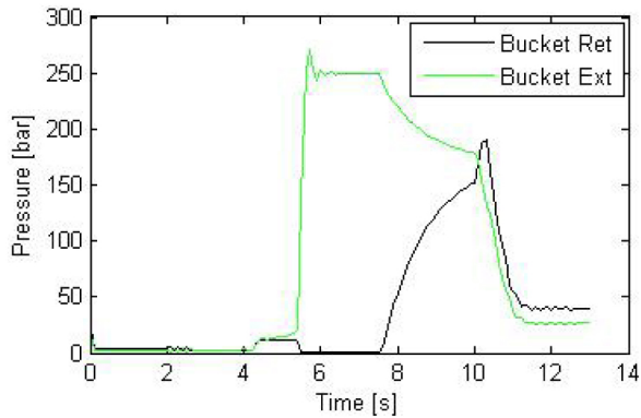
Fig. 25. Pressure in Bucket Actuator
